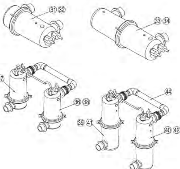
Canister Assembly (all models)
