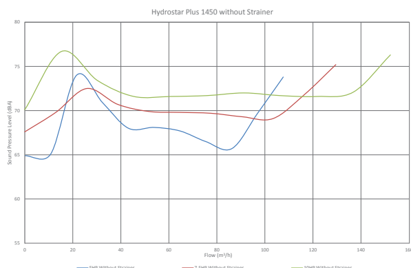
Noise Curve
