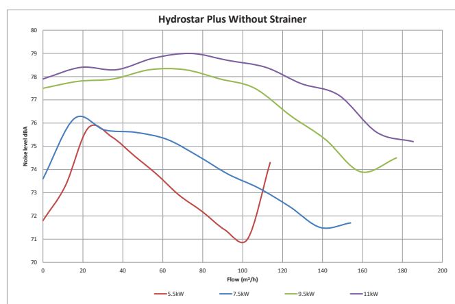
Noise Curve
