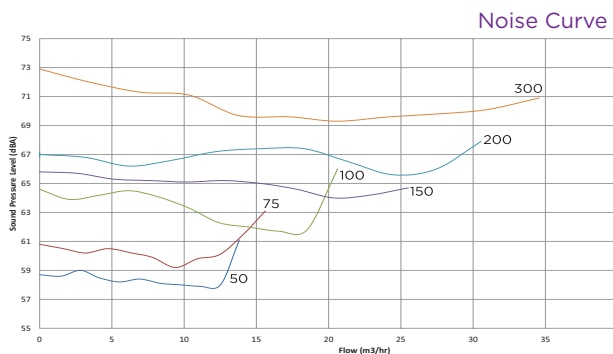
Noise Curve
