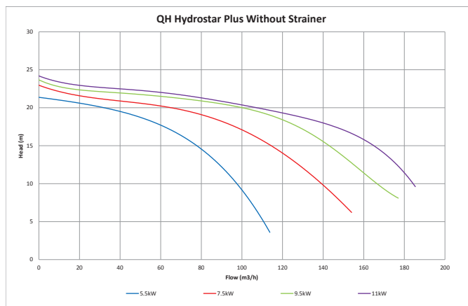
Flow Curve
