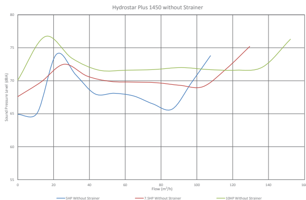
Flow Curve
