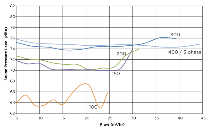
Noise Level
