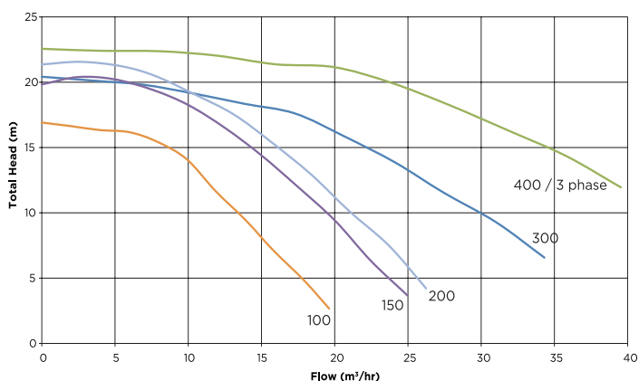
Flow Curve
