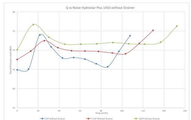
Noise Curve
