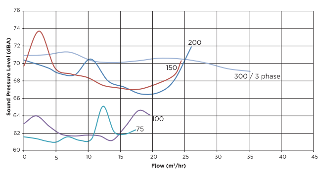
Noise Level
