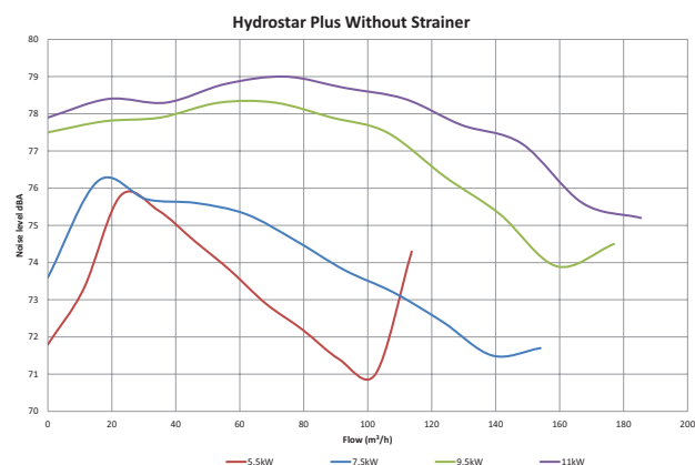
Noise Curve
