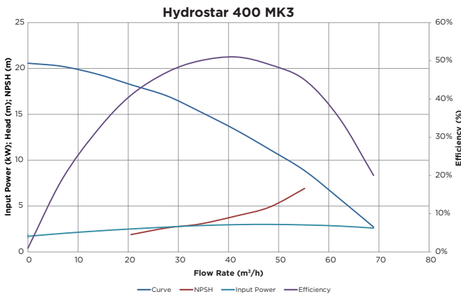
Flow Curve
