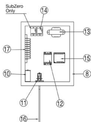
Electrical Box (all models)
