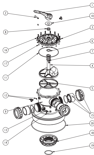
90mm Waterco Valve Top Mount
