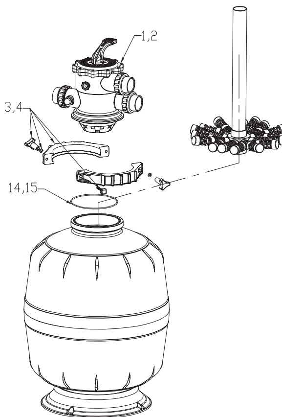
LATERAL CONFIGURATION FOR E600+ / 602+
