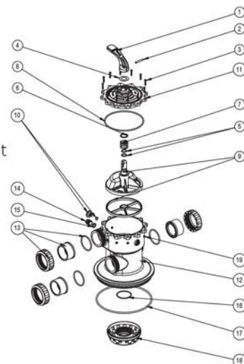
75mm Top Mount
