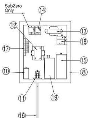
Electrical Box (all models)
