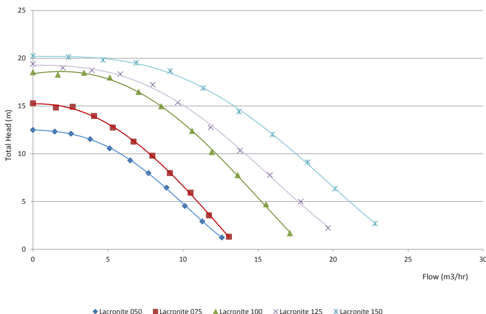
Flow Curve
