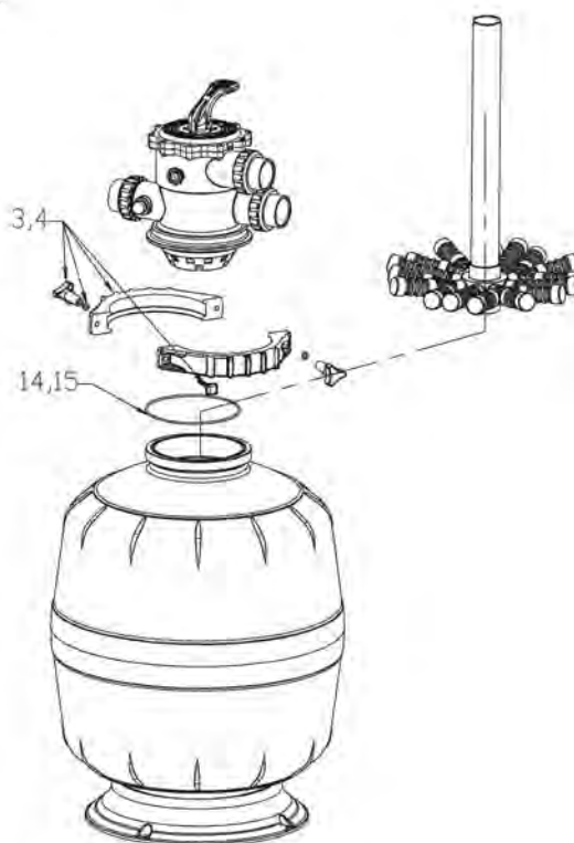
LATERAL CONFIGURATION FOR E600+ / E602+
