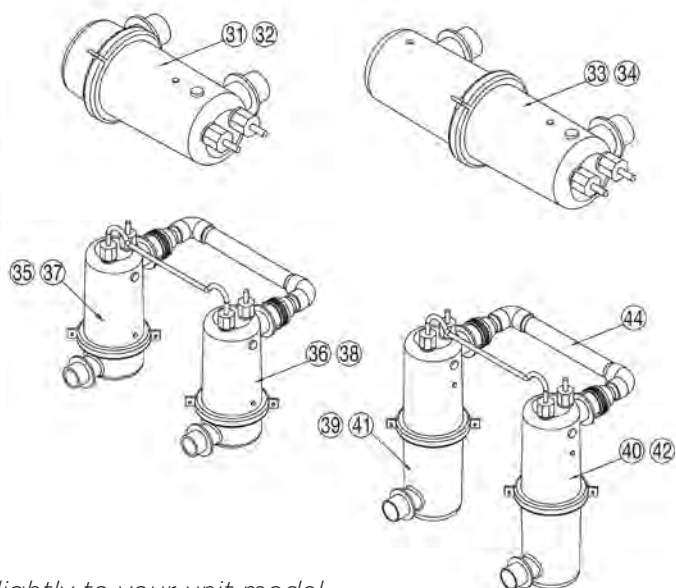
Canister Assembly (all models)
