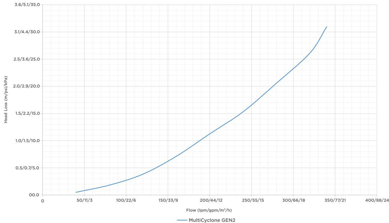
MultiCyclone 16 GEN2 total head loss curve
