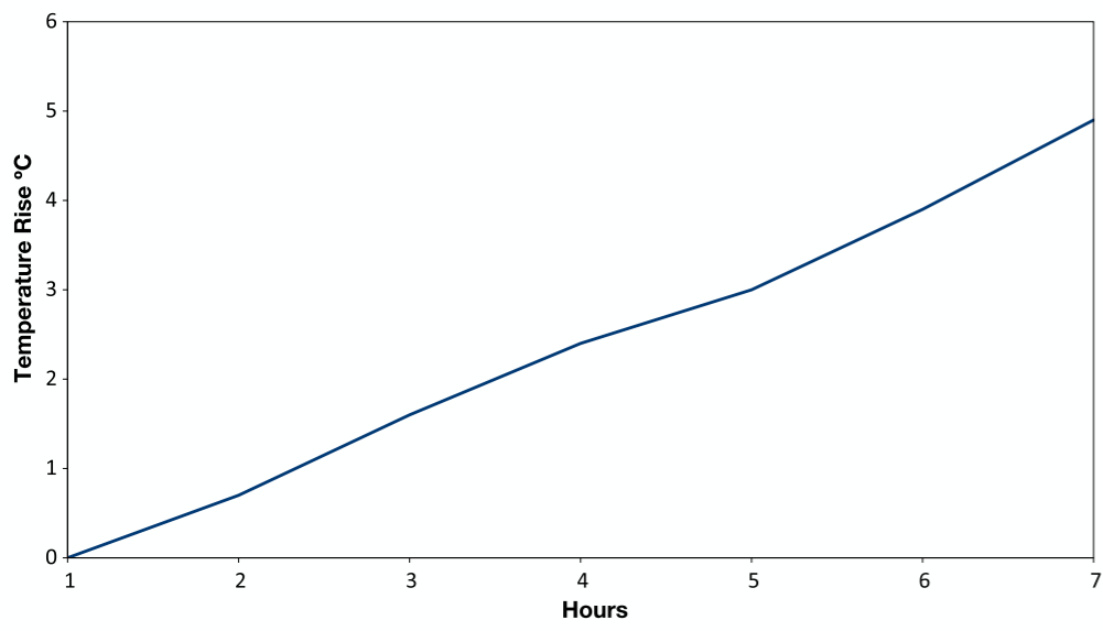
Electroheat Pro 100 Temperature Rise
